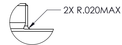
DETAIL C SCALE 4:1
